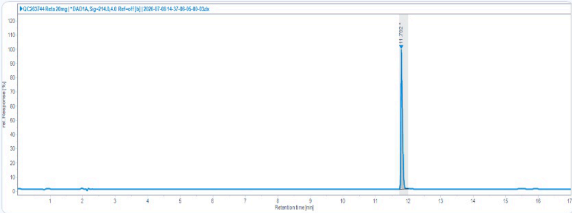
HPLC Chromatogram (Retention Time: 11.792 min)
