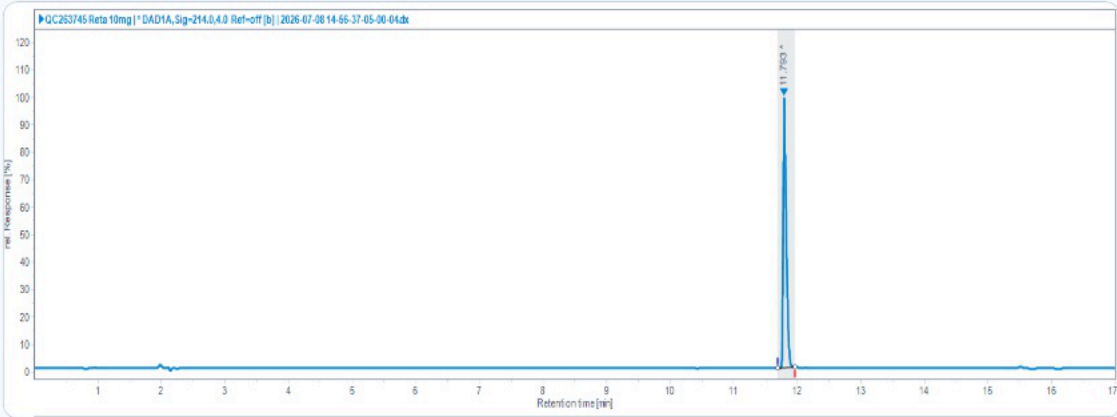
HPLC Chromatogram (Retention Time: 11.793 min)
